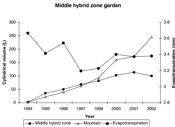
Figure 6. Mean cylindrical volume for middle hybrid and mountain seed source plants and average daily evapotranspiration in Nephi, Utah, during the years that the morphological data were collected from transplants in the gardens.
